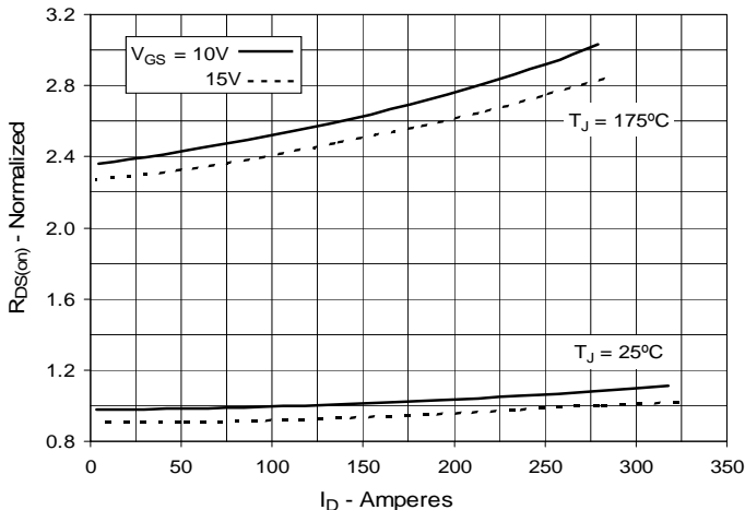
Fig. 5. R_{DS(on)} Normalized to I_D = 110A Value vs. Drain Current
